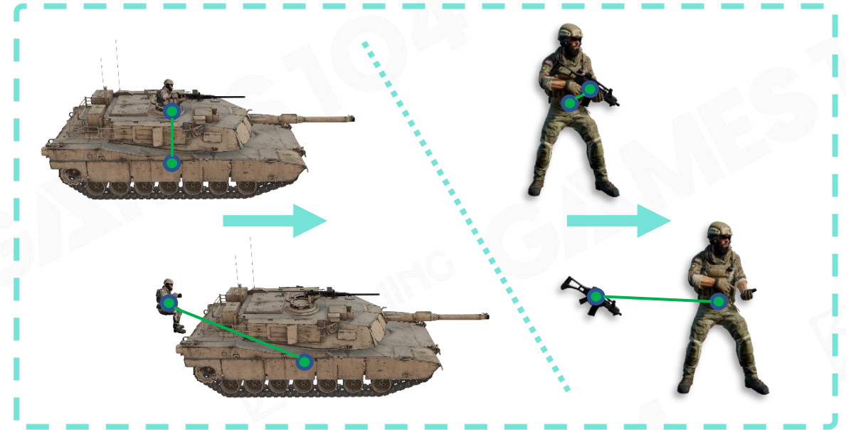
GO Bindings
