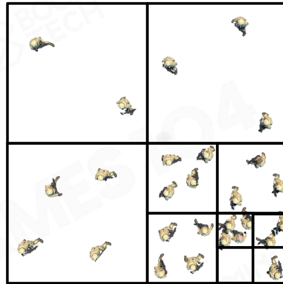
Quadtree
